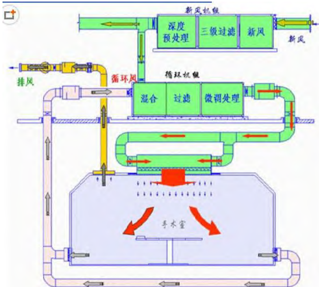
Air flow system
