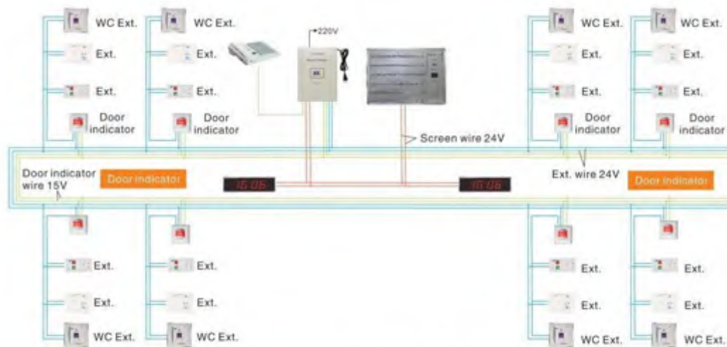
Wiring Diagram for BF Series Medical Calling System (with door indicator) Requirements for cables and wires: RVV2*0.75
